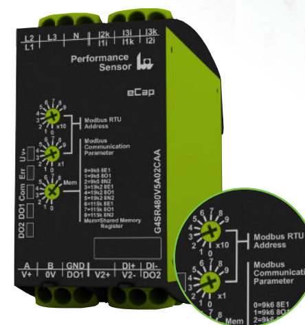
EASY ADJUSTABLE FRONT DIALS
